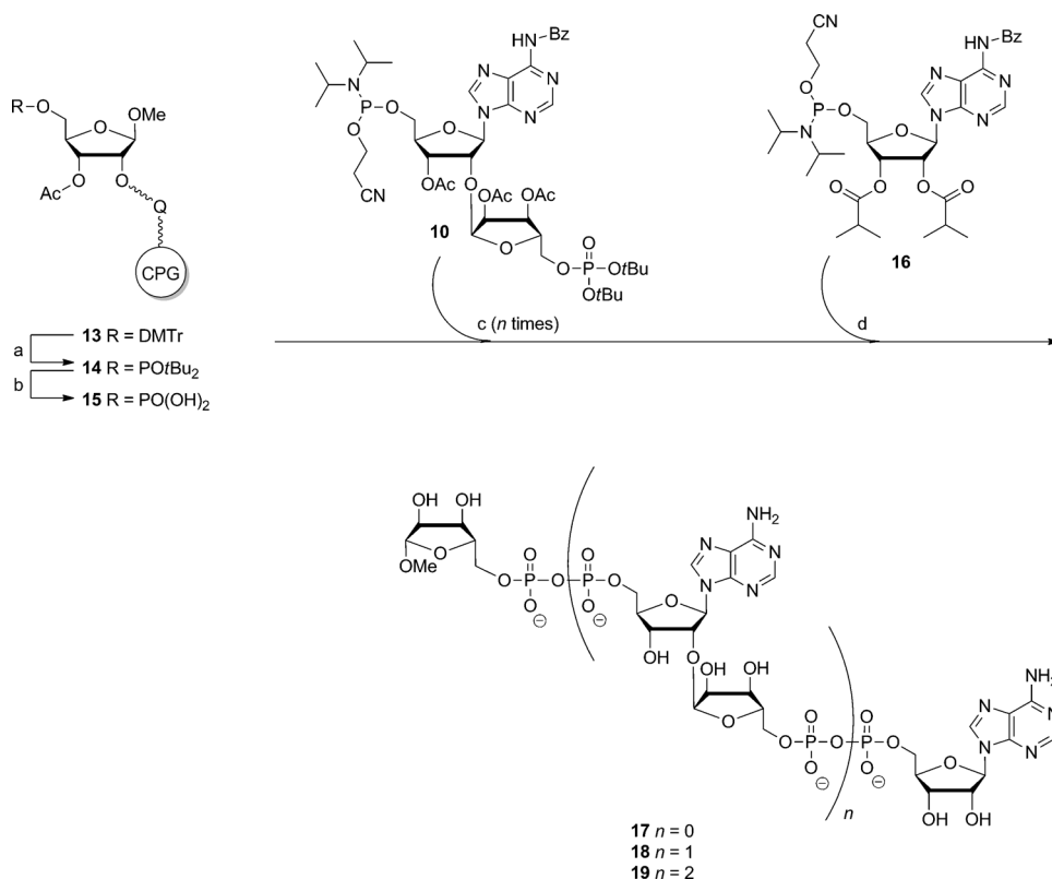
Scheme 4. Synthesis of the preloaded CPG resin and PAR oligomers ( n=0, 1 , and 2 ). a) i) TFA (5% v/v), \text{CH}_2\text{Cl}_2 ; ii) (\text{tBuO})_2\text{PNiPr}_2 , 1-Me-Im-HCl (0.3 M), 1-Me-Im (0.2 M), DMF; iii) CSO, MeCN; b) i) TFA (10% v/v), \text{CH}_2\text{Cl}_2 ; ii) pyridine/ \text{H}_2\text{O} (9:1, v/v); c) i) compound 10 (3 equiv), ETT (10 equiv), MeCN (2 \times ); ii) CSO (100 equiv), MeCN (2 \times ); iii) DBU (100 equiv), DMF, (2 \times ); iv) HCl (5 equiv), HFIP (4 \times ); v) pyridine (10% v/v), acetonitrile (2 \times ); d) i) compound 16 (3 equiv), [16] ETT (10 equiv), MeCN (2 \times ); ii) CSO (100 equiv), MeCN (2 \times ); iii) DBU (100 equiv), DMF (2 \times ); iv) \text{NH}_4\text{OH} (35%).
